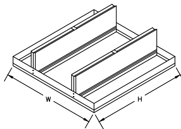
UL LISTED RADIATION FIRE DAMPER MODEL # 615
