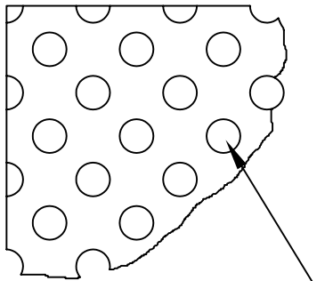
Perforated face plate 3/16" diameter holes 1/4" staggered centers
