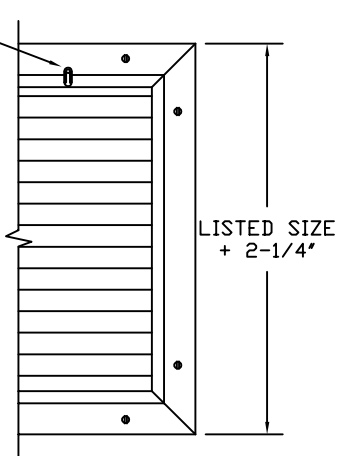
MODEL RAF/GS (FOR NOM. DUCT SIZE)
