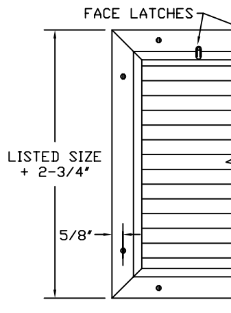
MODEL RAF/FS (FOR NOM. FILTER SIZE)
