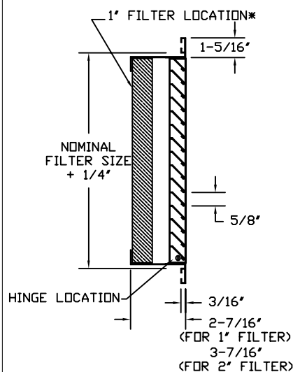
BORDER OPTION TYPE TB (LAY-IN)
