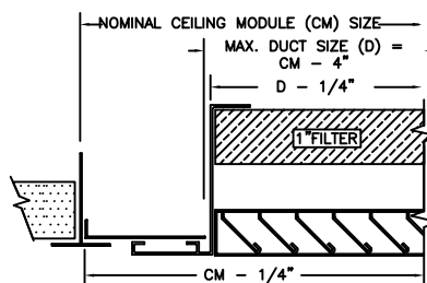
BORDER OPTION TYPE TB (LAY-IN)
